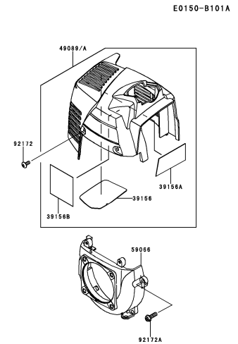
B-05 COOLING-EQUIPMENT
