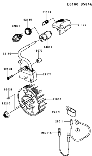
B-06 ELECTRIC-EQUIPMENT
