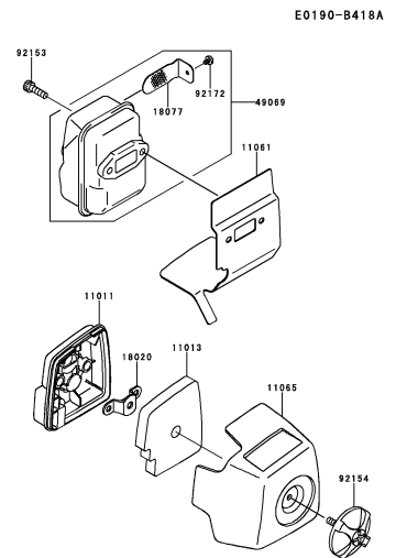
B-08 AIR-FILTER/MUFFLER
