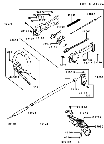
C-03 PIPE/HANDLE/GUARD
