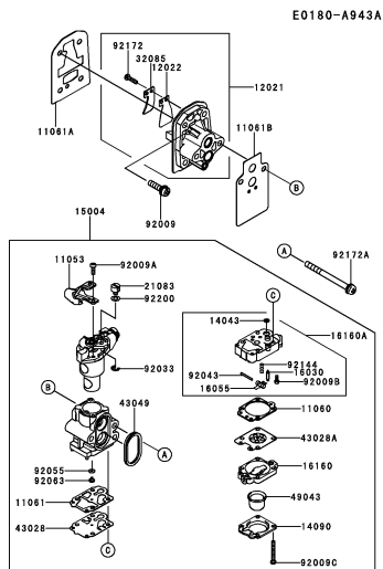
B-07 CARBURETOR
