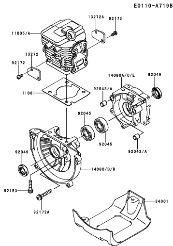
B-03 CYLINDER/CRANKCASE
