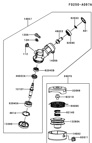
C-06 CASE/CUTTER
