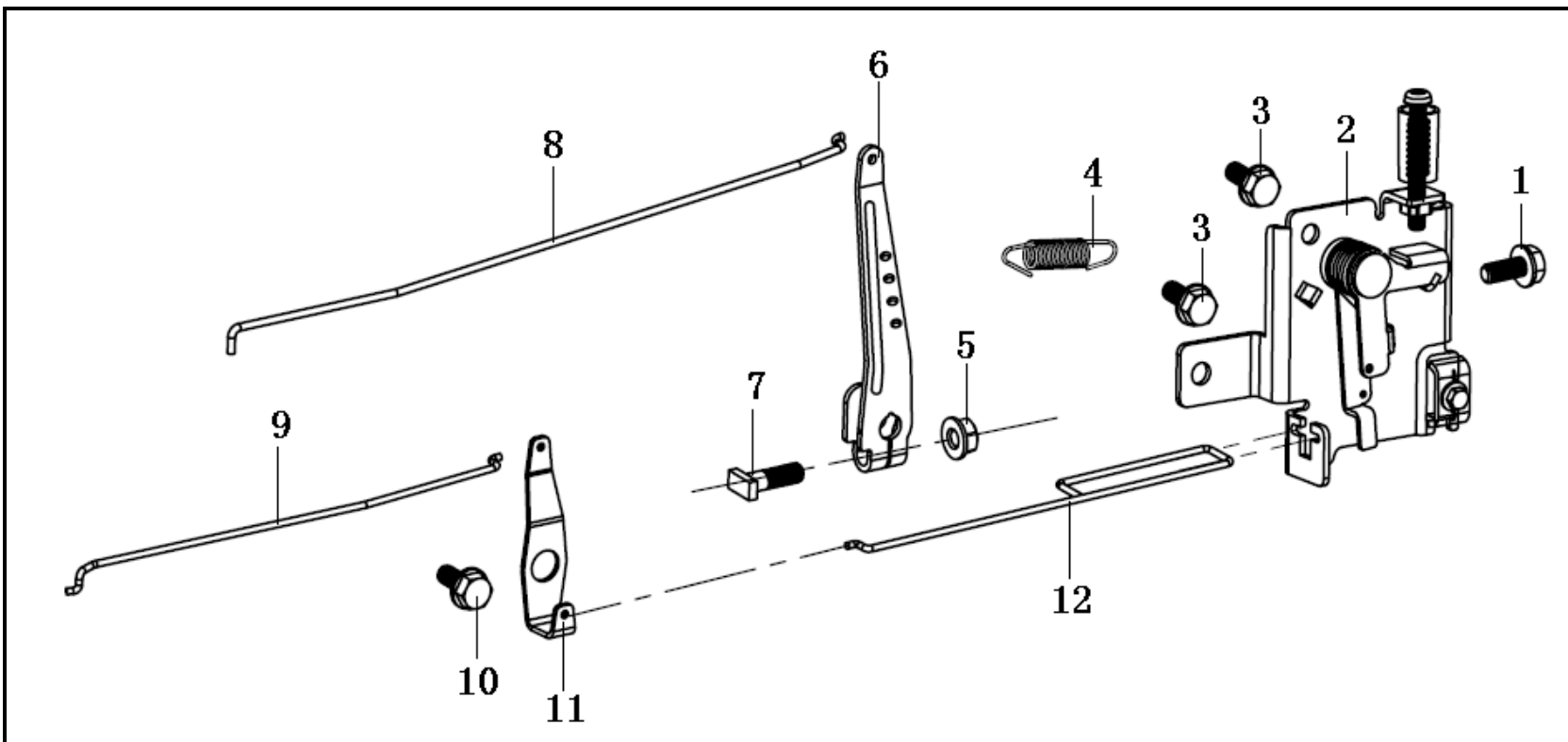
(Governor)
