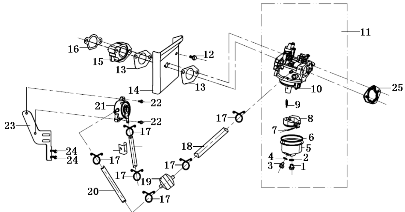
(Carburetor With Pump)
