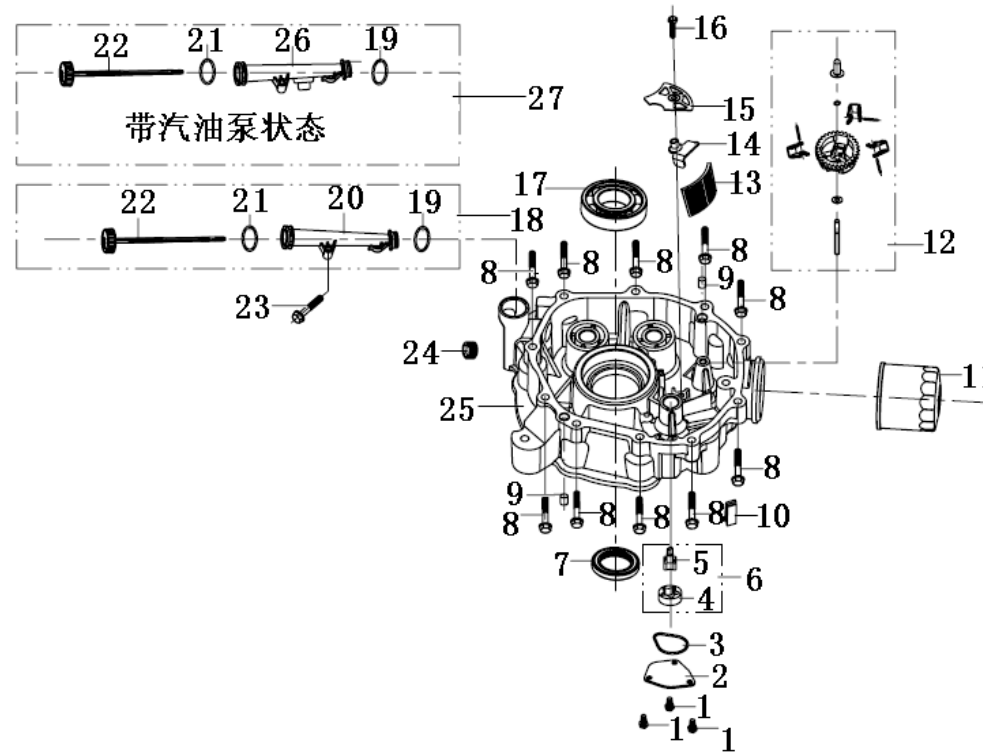
(Crankshaft Cover)
