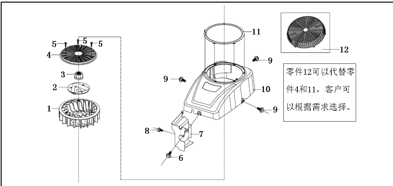
(Blower Housing)
