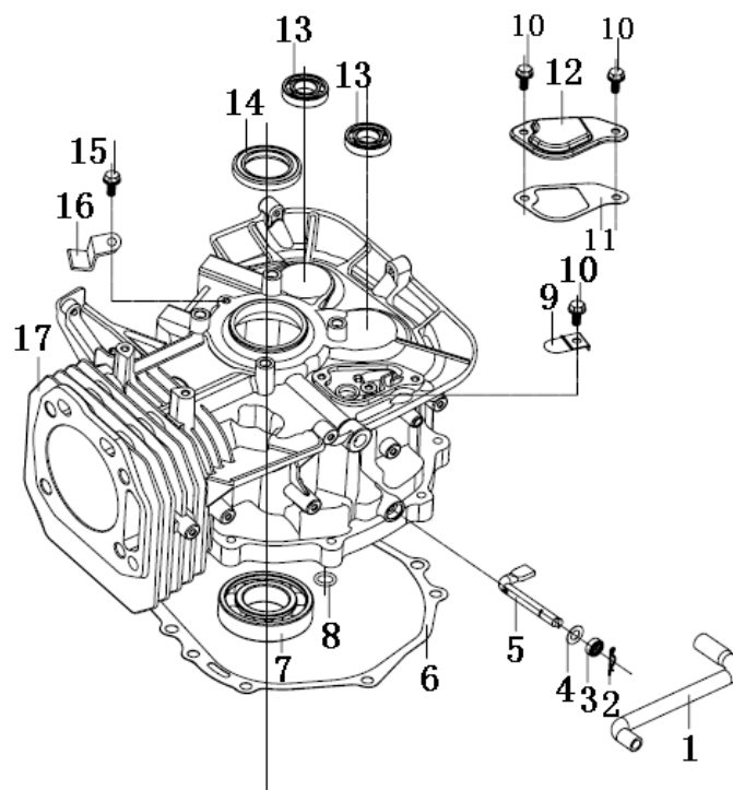
(Crankcase)
