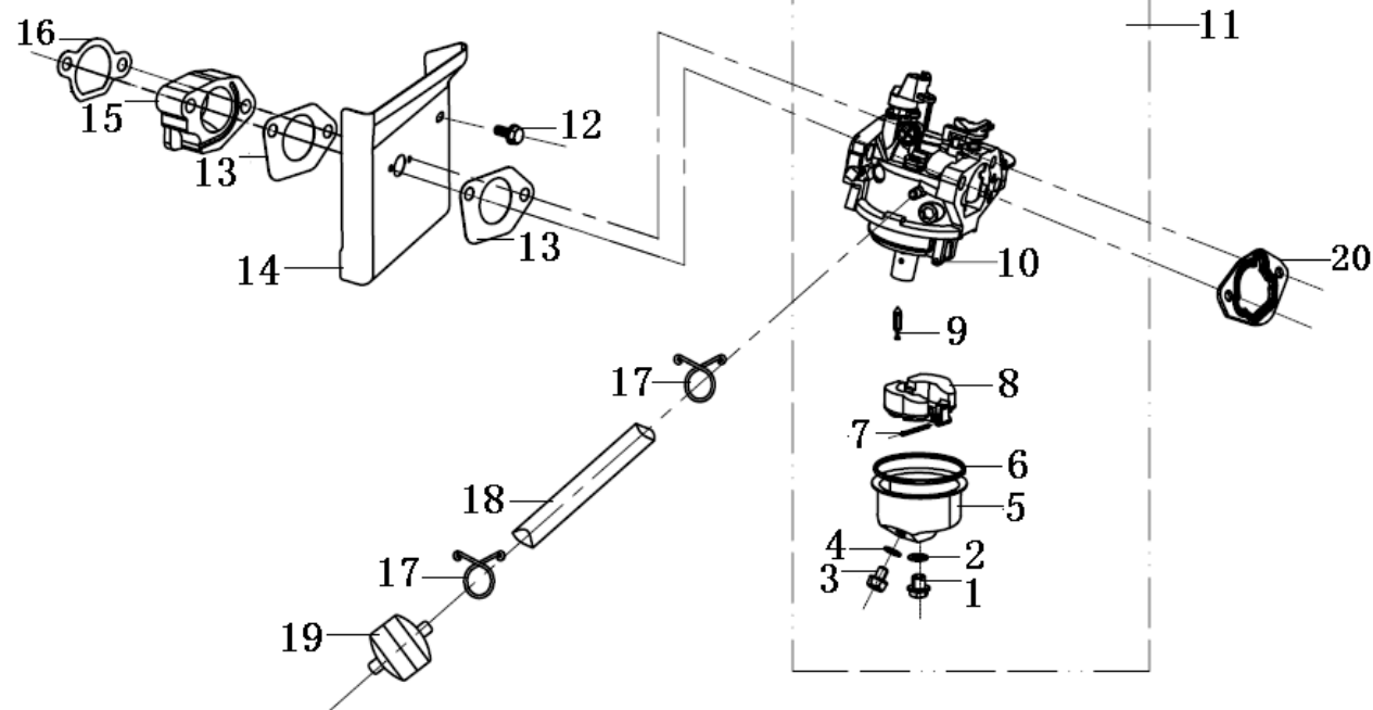
(Carburetor)
