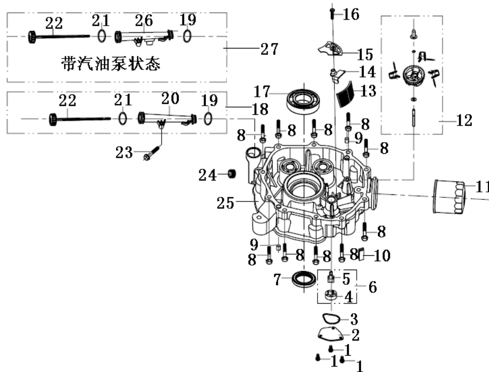
(Crankshaft Cover)
